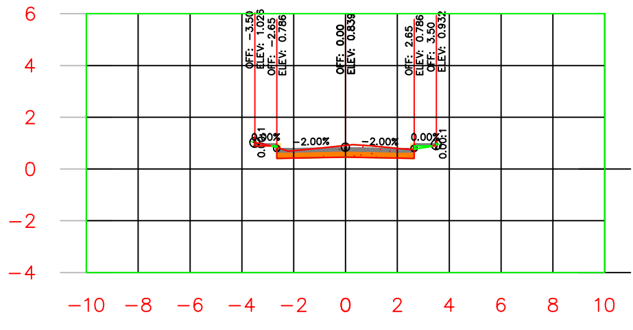
K0+150.00
