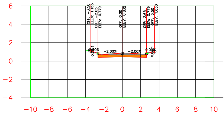
K0+165.00
