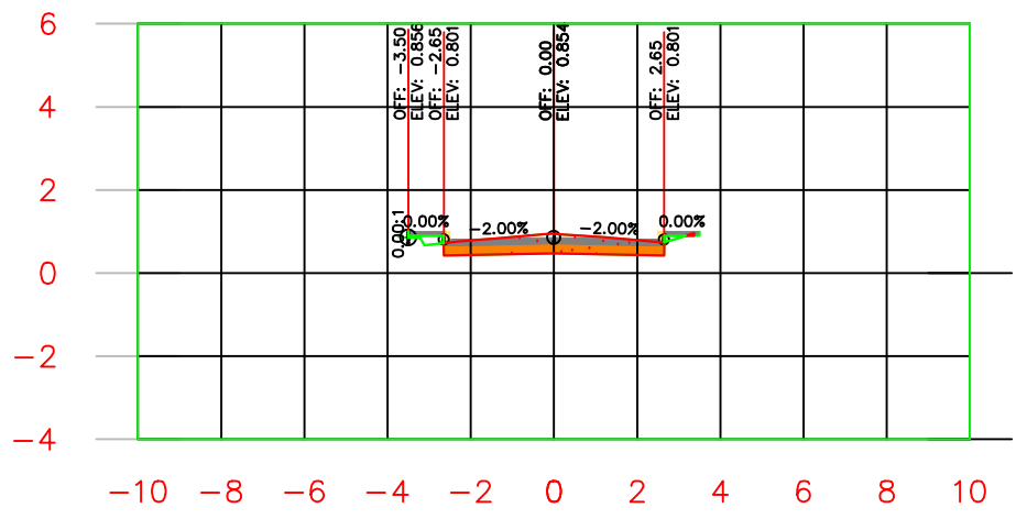
K0+120.00
