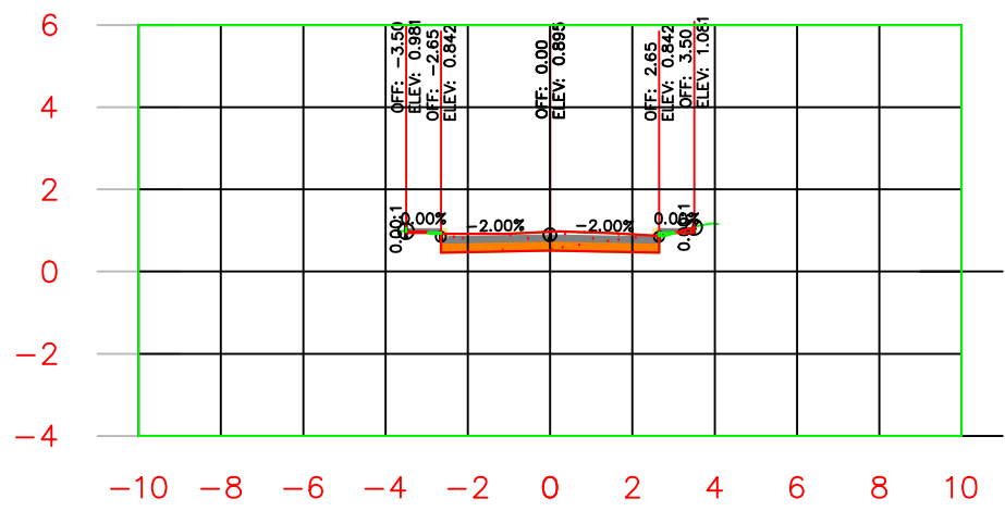
K0+035.00
