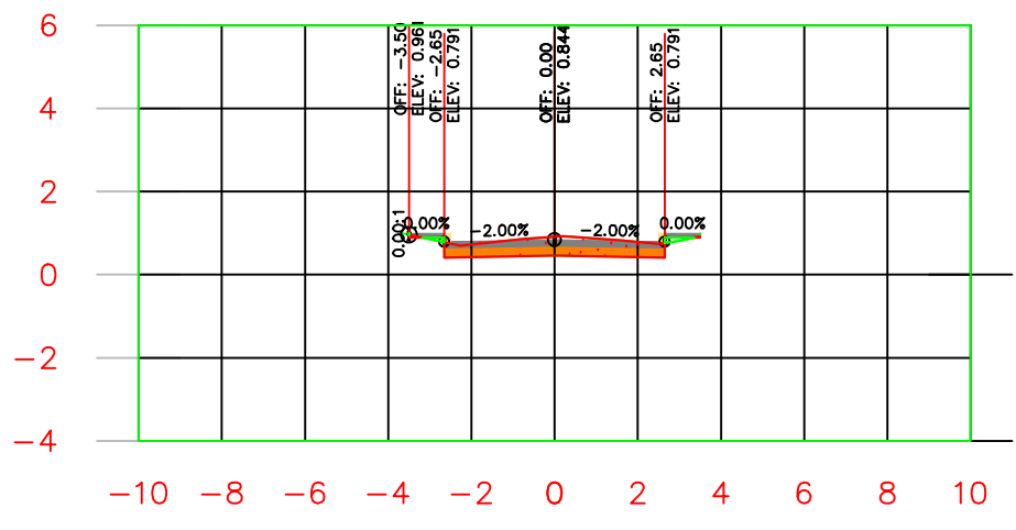
K0+140.00
