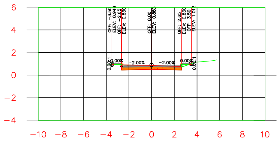
K0+060.00
