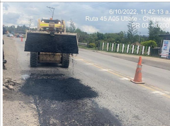
Tapahuecos PR3+0000 a PR10+0750 (06/10/22)
