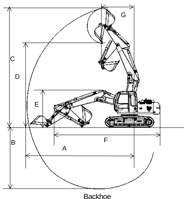
Backhoe
