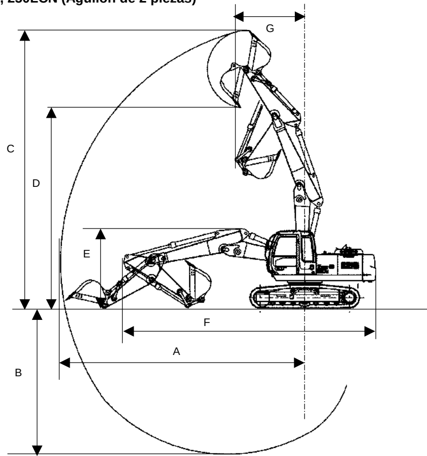
Backhoe
