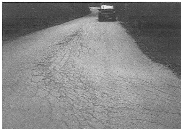
PR 2+000
