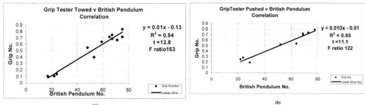
Figure 24. Correlation of British Pendulum Number to GripTester (a – towed, b – pushed), (16)
