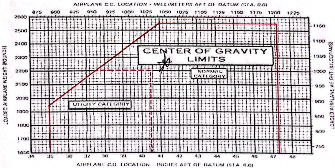
Figure B-8. Center of Gravity Limits
