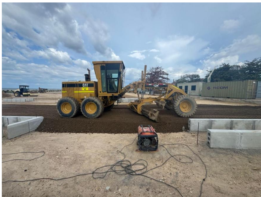
Base granular
