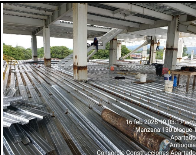
Instalacion steel deck Torre Medica
