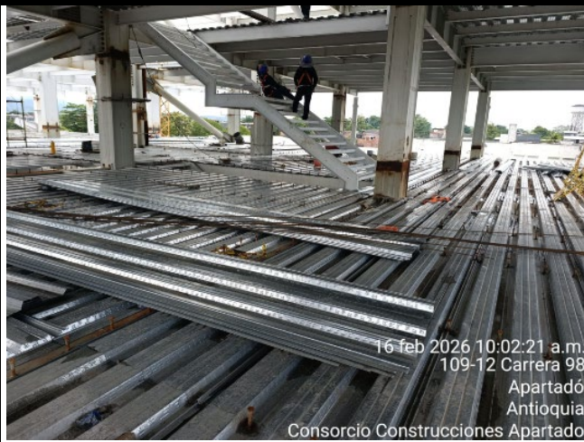
Instalacion steel deck Torre Medica
