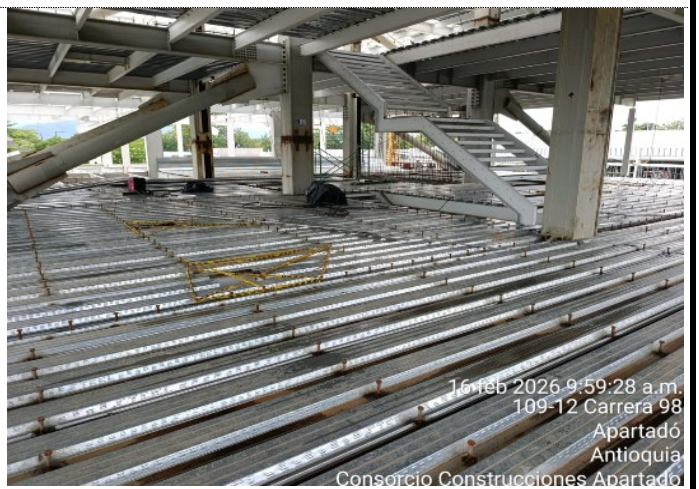
Instalacion steel deck Torre Medica
