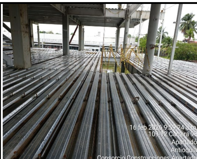
Instalacion steel deck Torre Medica
