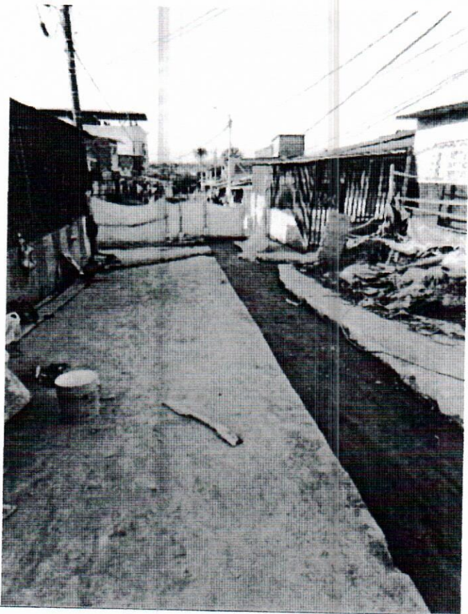
Subbase granular
