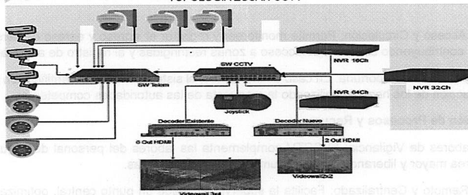
TOPOLOGIA ECSAN CCTV
