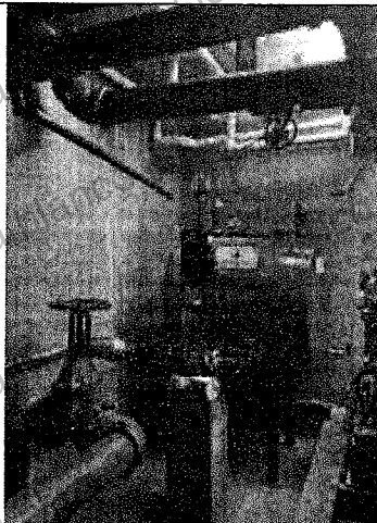
INSTALACION BOMBA JOCKEY 1.5 HP
