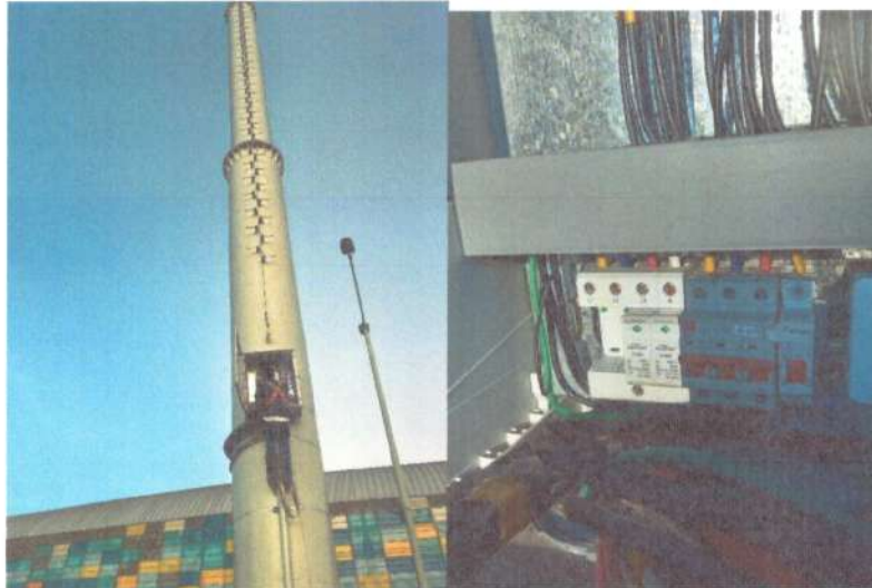
MASTIL No. 4
