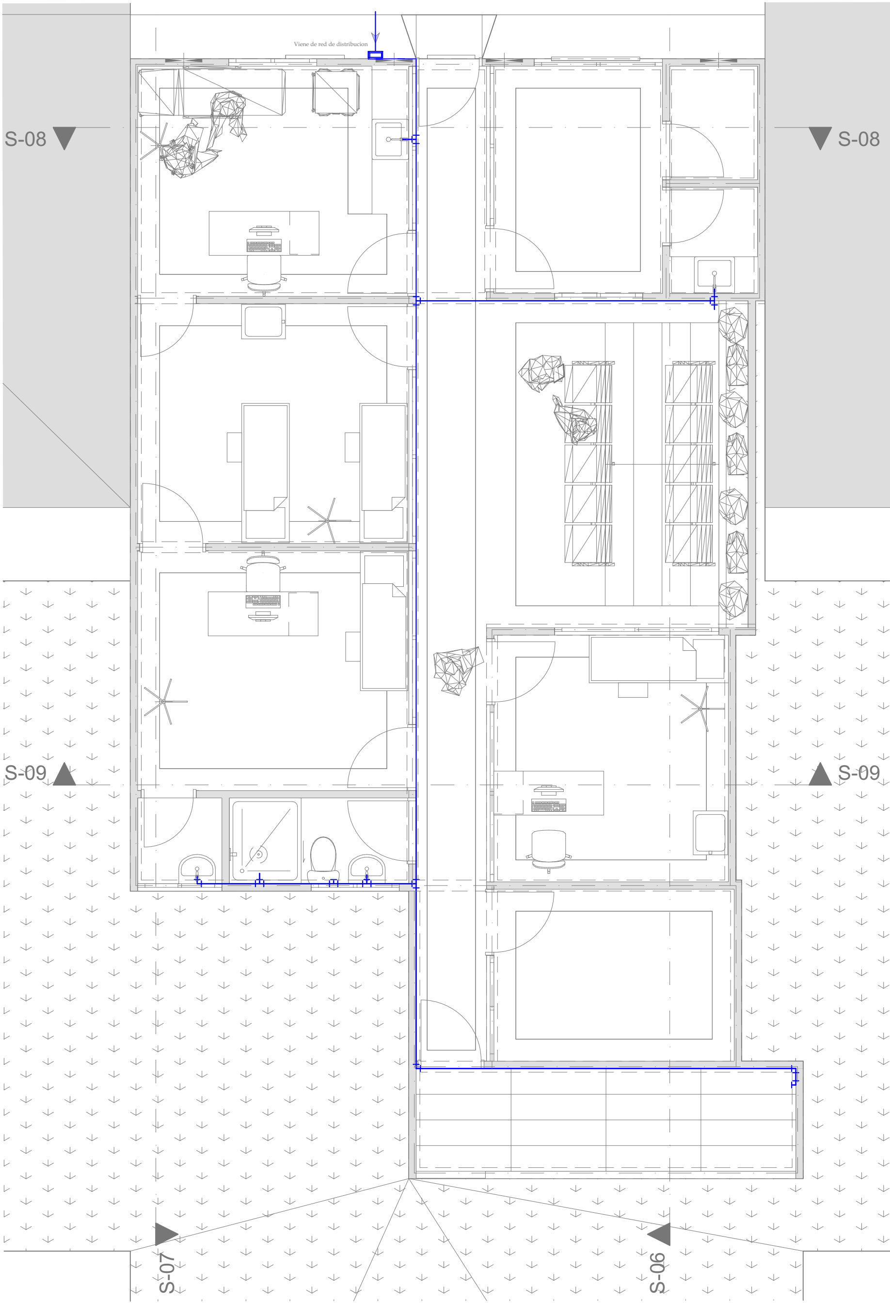
0. Ground Floor (18) 1:50
