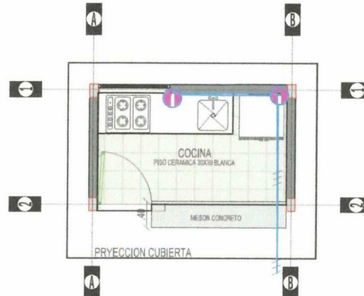
PLANTO TOMACORRIENTE
