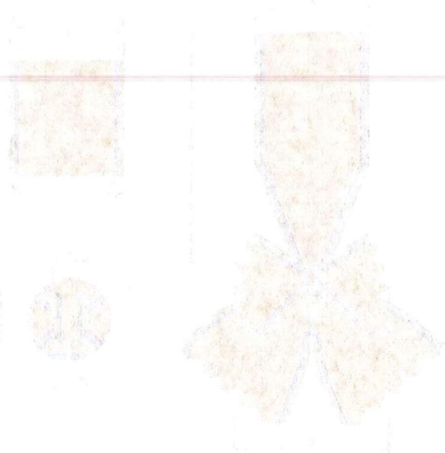
Figure 2. Banding patterns of the DNA fragments
