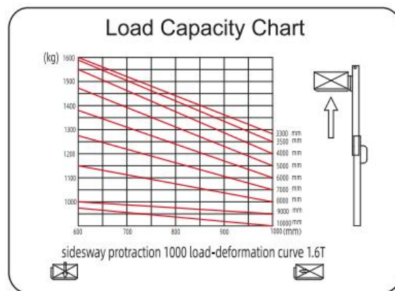
CQDH20C (double scissors)
