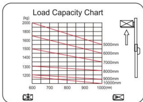
CQDH20C (single scissor)
