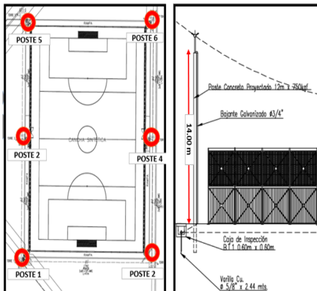
Salida Parcial Electrica (2 THHN No.10 + 1 THHN No.12)
