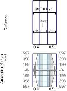
VCPPrim10 / Base F'c=21Mpa Fy=420Mpa d'=60mm
