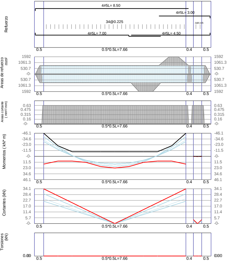
VCPPrim9 / Base F'c=21Mpa Fy=420Mpa d'=60mm
