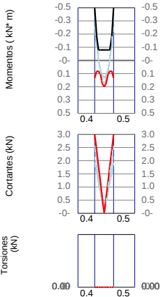
VCPPrim9 / Base F'c=21Mpa Fy=420Mpa d'=60mm
