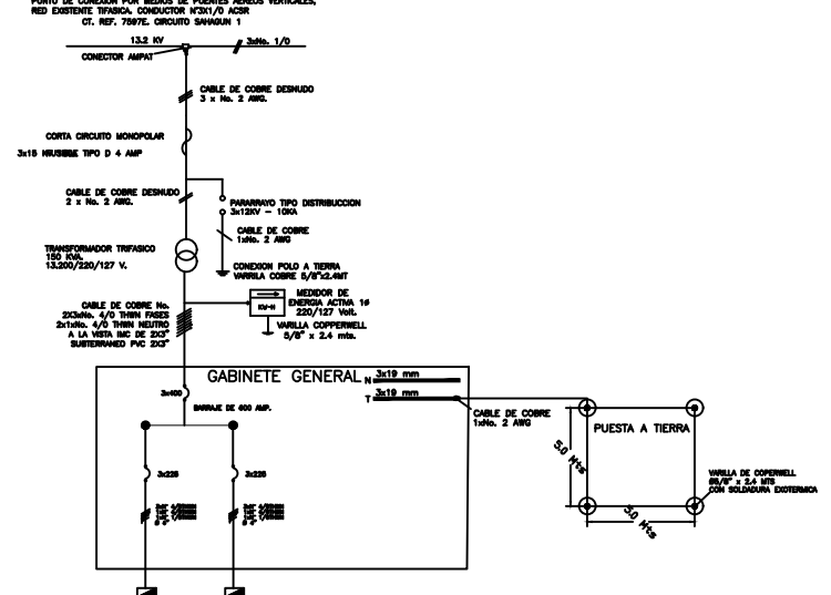
DIAGRAMA UNIFILAR
