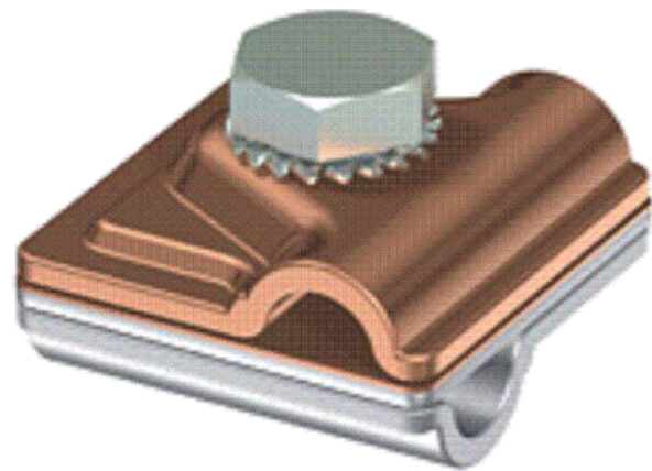
DETALLE N°16 CONECTOR VARIABLE BIMETALICO REF 249 ZV
