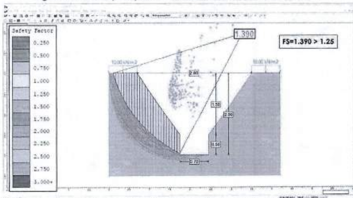
Figura 23. FS Bishop simplified – Excavación colector talud 0.70H:1V
