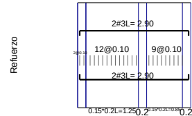
VP9 / Story1 F'c=21Mpa Fy=420Mpa d'=60mm
