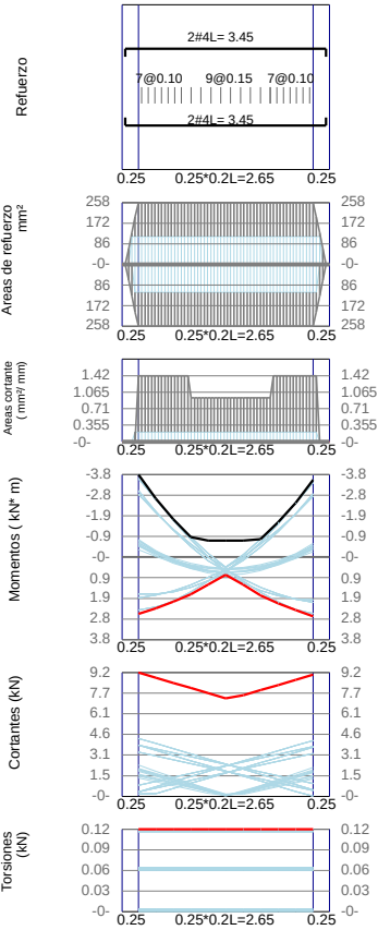
VP7 / Story1 F'c=21Mpa Fy=420Mpa d'=60mm
