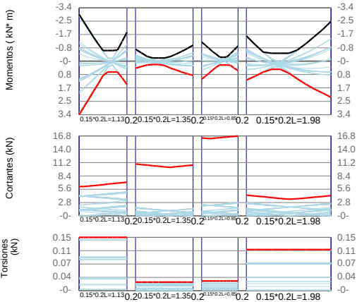
VP9 / Story1 F'c=21Mpa Fy=420Mpa d'=60mm
