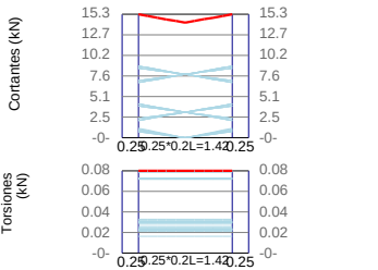
VP7 / Story1 F'c=21Mpa Fy=420Mpa d'=60mm
