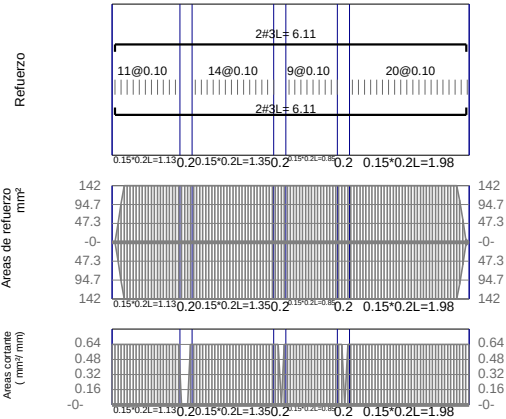
VP8 / Story1 F'c=21Mpa Fy=420Mpa d'=60mm
