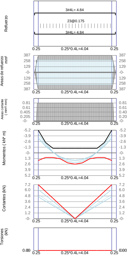
VCAnd1 / Base F'c=21Mpa Fy=420Mpa d'=60mm
