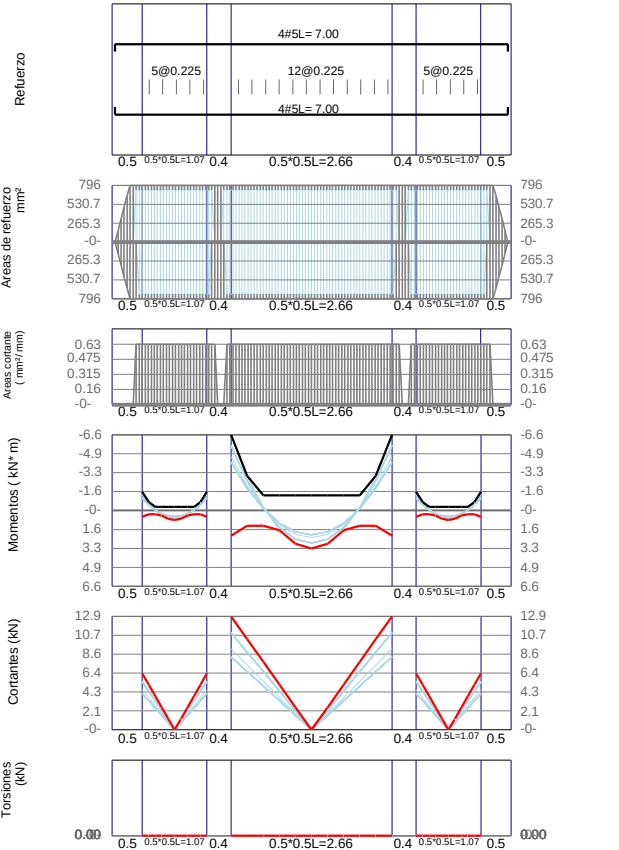
VCB-7 / Base F'c=21Mpa Fy=420Mpa d'=60mm
