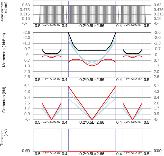
VCB-9 / Base F'c=21Mpa Fy=420Mpa d'=60mm
