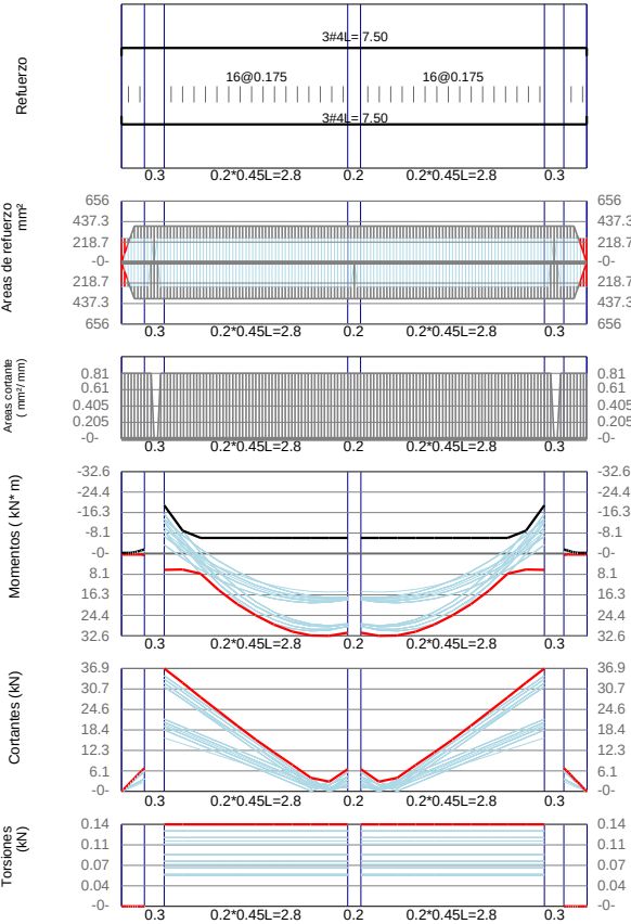
VB-7 / Story1 F'c=21Mpa Fy=420Mpa d'=60mm
