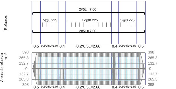
VCB-8 / Base F'c=21Mpa Fy=420Mpa d'=60mm
