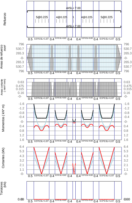
VCB-9 / Base F'c=21Mpa Fy=420Mpa d'=60mm
