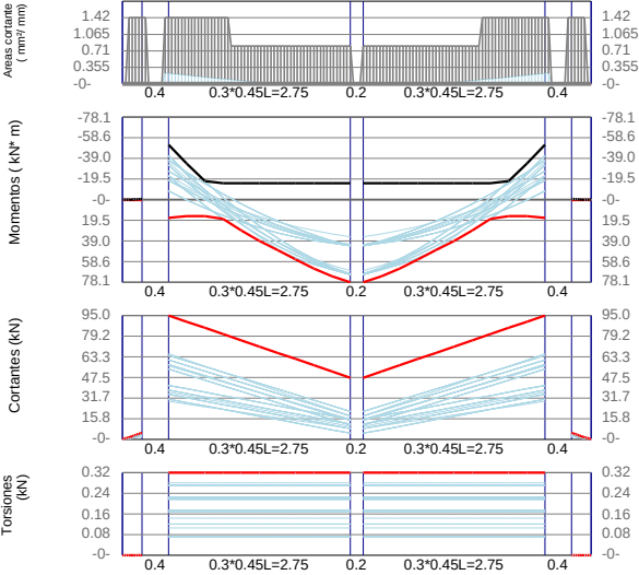
VB-8 / Story1 F'c=21Mpa Fy=420Mpa d'=60mm
