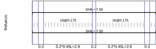
VB-9 / Story1 F'c=21Mpa Fy=420Mpa d'=60mm
