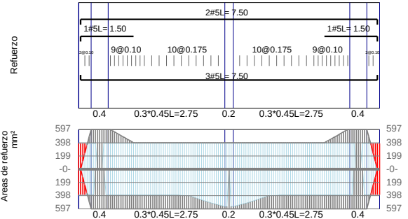
VB-7 / Story1 F'c=21Mpa Fy=420Mpa d'=60mm
