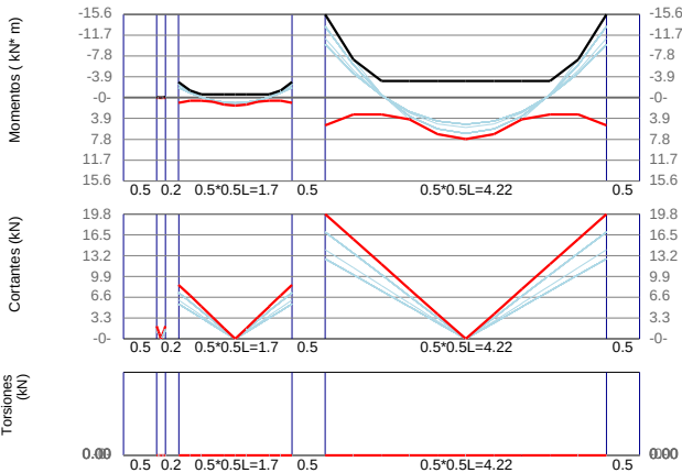
VCB-7 / Base F'c=21Mpa Fy=420Mpa d'=60mm
