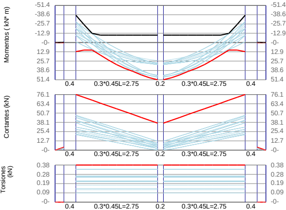
VB-6 / Story1 F'c=21Mpa Fy=420Mpa d'=60mm
