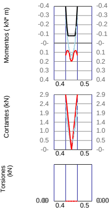
VC2-18 / Base F'c=21Mpa Fy=420Mpa d'=60mm
