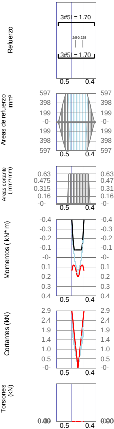
VC2-18 / Base F'c=21Mpa Fy=420Mpa d'=60mm
