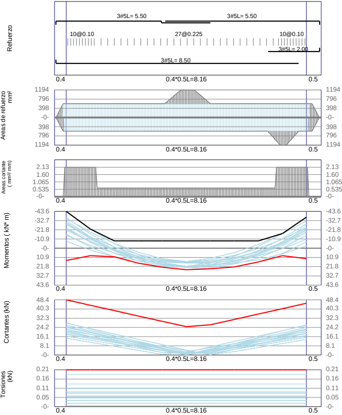
VBb2 / Story1 F'c=21Mpa Fy=420Mpa d'=60mm
