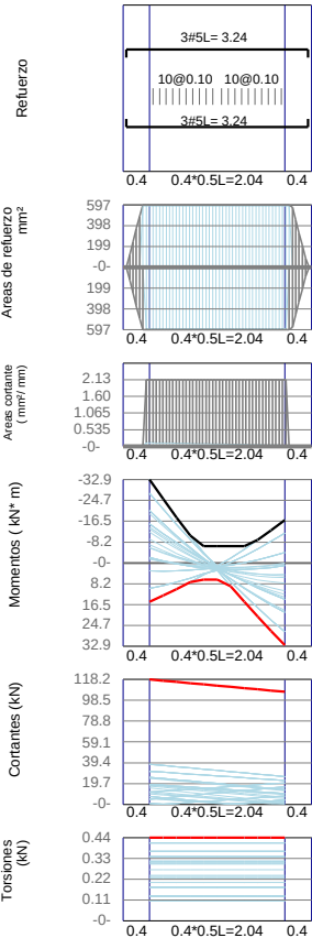
VBb4 / Story1 F'c=21Mpa Fy=420Mpa d'=60mm
