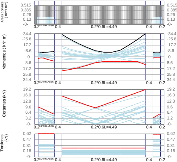
VBB12 / Story2 F'c=21Mpa Fy=420Mpa d'=60mm
