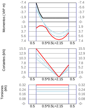
VCBb10 / Base F'c=21Mpa Fy=420Mpa d'=60mm
