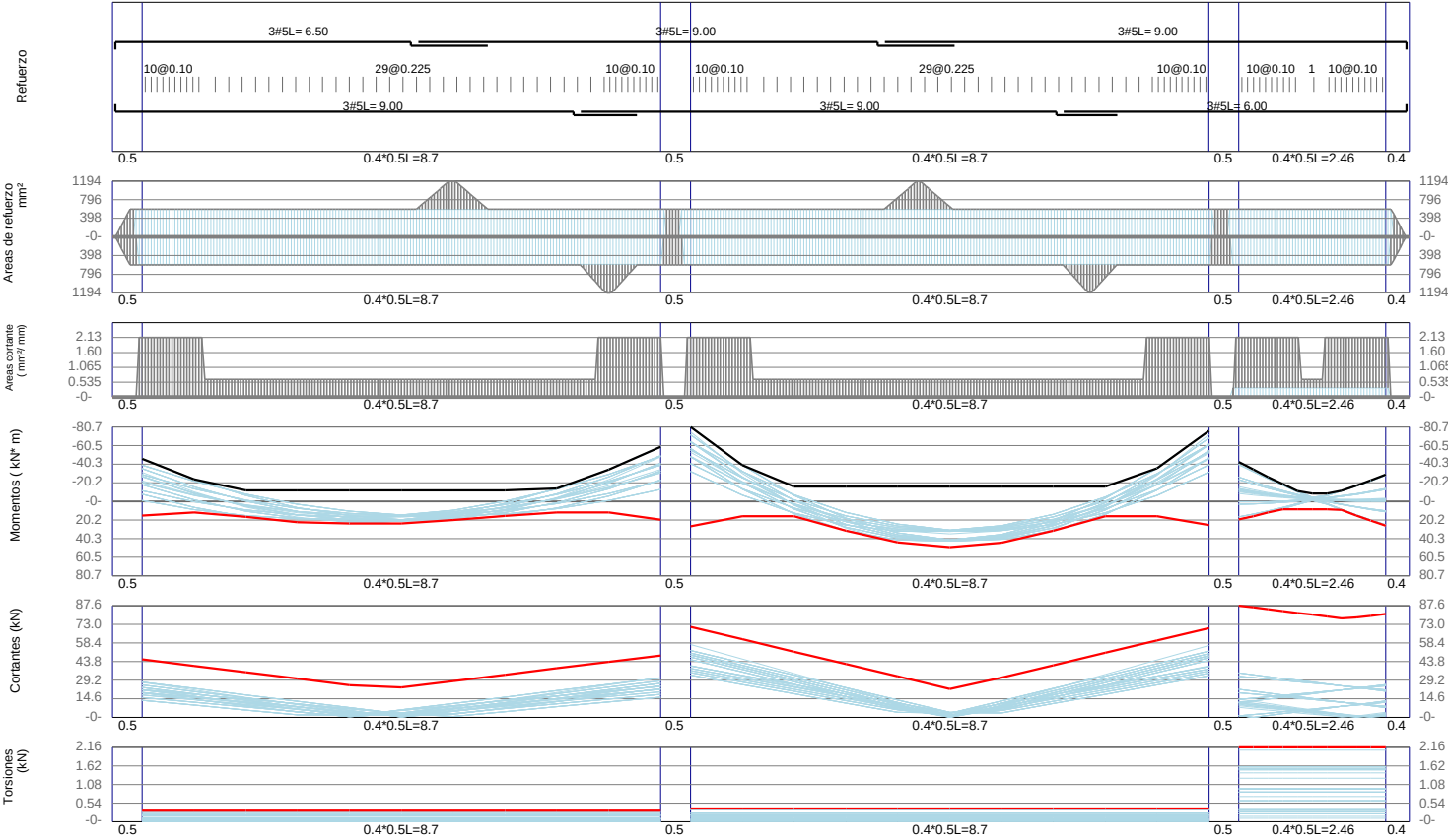
VBb2 / Story1 F'c=21Mpa Fy=420Mpa d'=60mm
