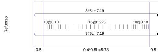
VBb5 / Story1 F'c=21Mpa Fy=420Mpa d'=60mm
