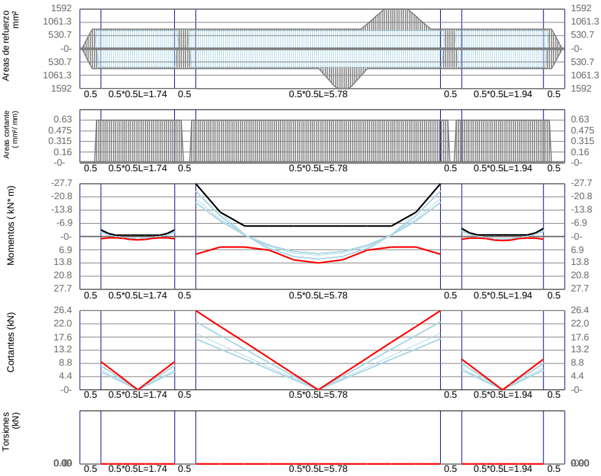
VBb1 / Story1 F'c=21Mpa Fy=420Mpa d'=60mm
