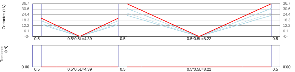
VCBb8 / Base F'c=21Mpa Fy=420Mpa d'=60mm
