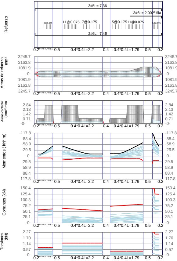
VBb15 / Story2 F'c=21Mpa Fy=420Mpa d'=60mm
