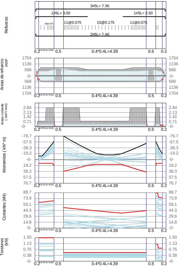
VBB12 / Story2 F'c=21Mpa Fy=420Mpa d'=60mm
